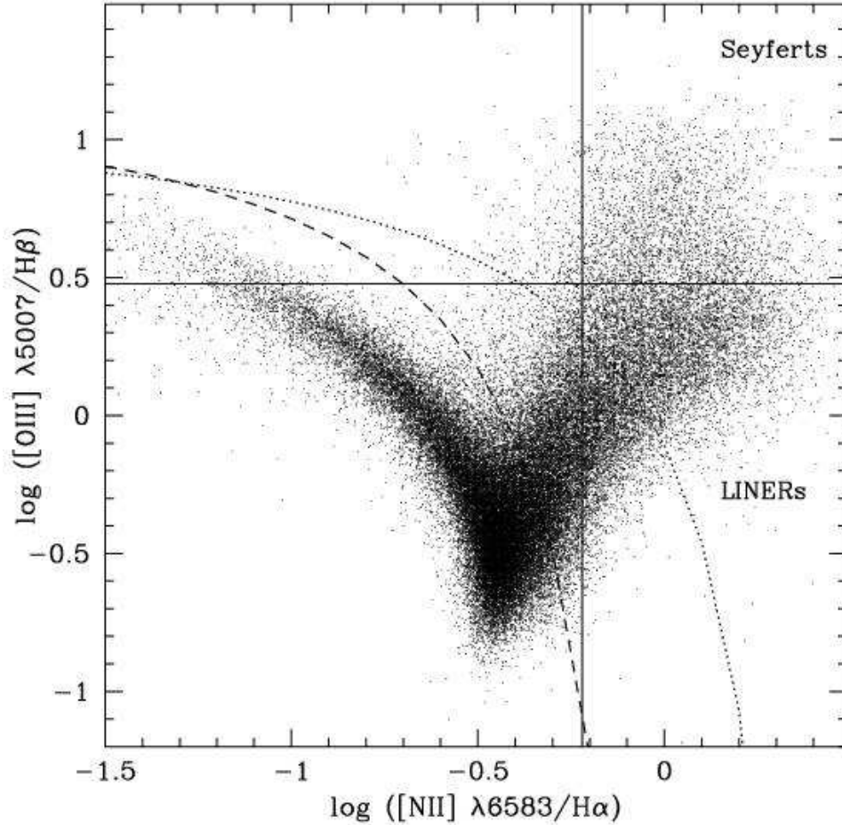
Figure 1: An example of a BPT (Baldwin, Phillips & Terlevich 1981) diagram in which we plot the emission line flux ratio [\text{OIII}]/\text{H}\beta versus the ratio [\text{NII}]/\text{H}\alpha for all the galaxies in our sample where all four lines are detected with S/N > 3 (55,757 objects). The dotted curve shows the demarcation between starburst galaxies and AGN defined by Kewley et al (2001). The dashed curve shows our revised demarcation (equation 1). A total of 22,623 galaxies lie above dashed curve. Seyfert galaxies are often defined to have [\text{OIII}]/\text{H}\beta > 3 and [\text{NII}]/\text{H}\alpha > 0.6 , and LINERs to have [\text{OIII}]/\text{H}\beta < 3 and [\text{NII}]/\text{H}\alpha > 0.6 . Our sample includes 2537 Seyferts and 10,489 LINERs according to this definition.
